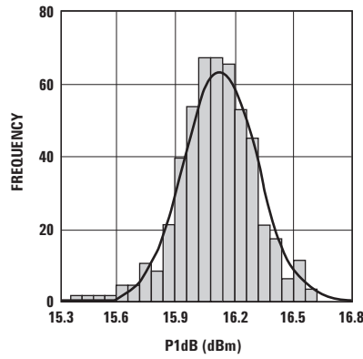
Figure 2. P1dB Distribution.
