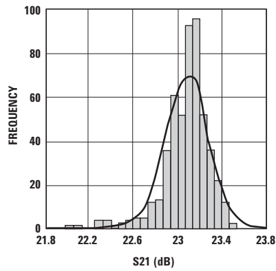
Figure 1. S21 Distribution.
